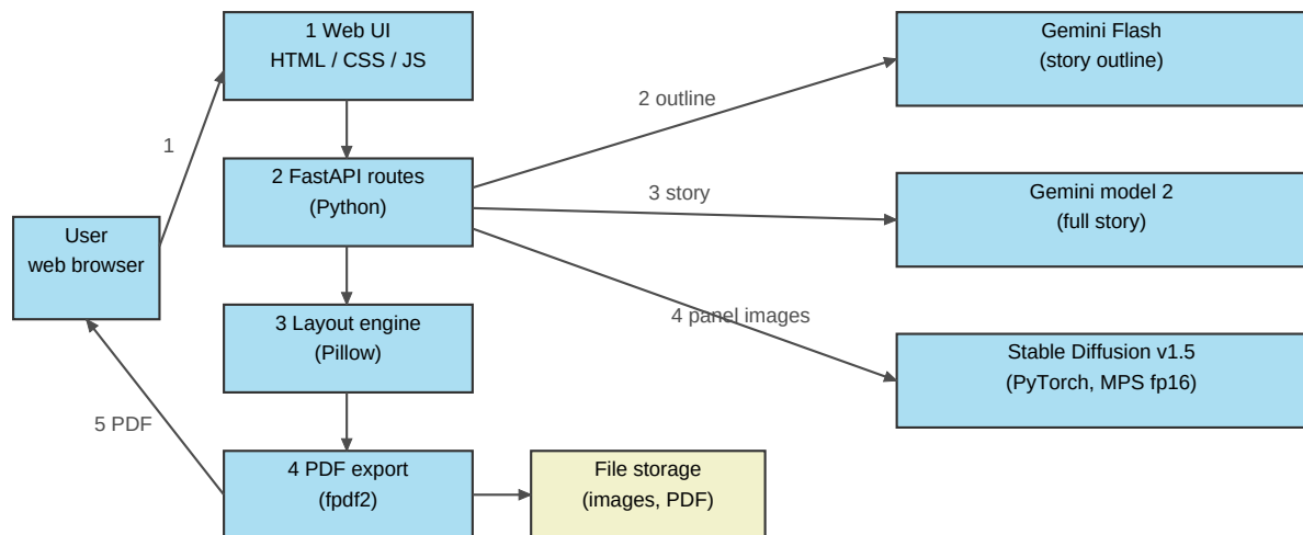
Figure 1: Architecture and data flow of ComicCraft (AI comic story creator)
